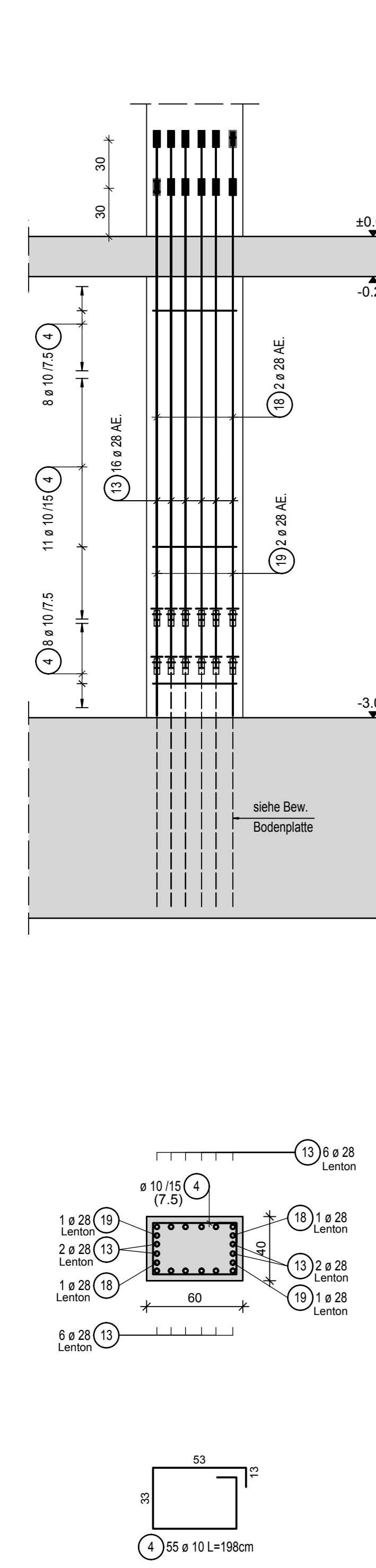
Stb. Stütze b/h=60/40cm (C35/45, XD3, XF1, WF) Pos. S19
