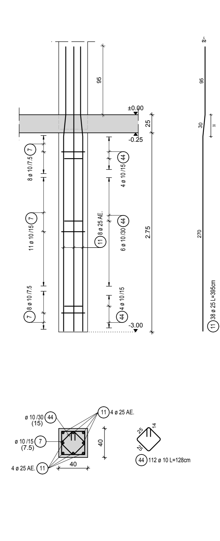
4x Stb. Stütze b/h=40/40cm (C35/45, XD3, XF1, WF) Pos. S17, Pos. S21 Pos. S22, Pos. S24
