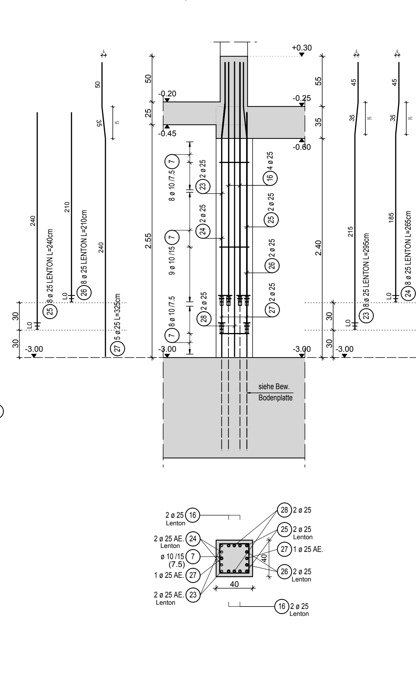
4x Stb. Stütze b/h=40/40cm (C35/45, XD3, XF1, WF) Pos. S42, Pos. S43 Pos. S44, Pos. S45
