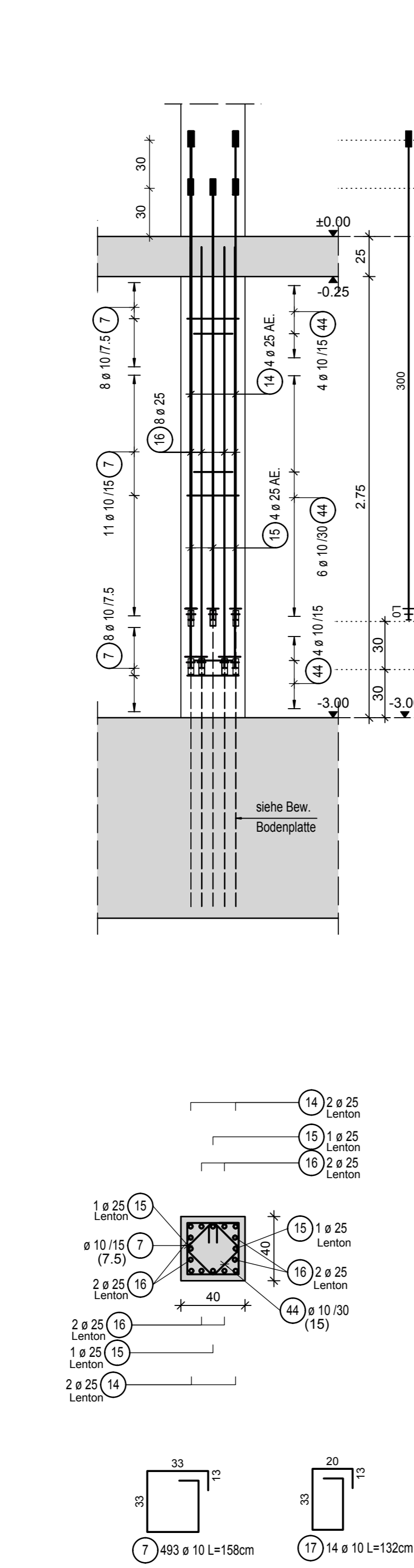
2x Stb. Stütze b/h=40/40cm (C35/45, XD3, XF1, WF) Pos. S18, Pos. S20
