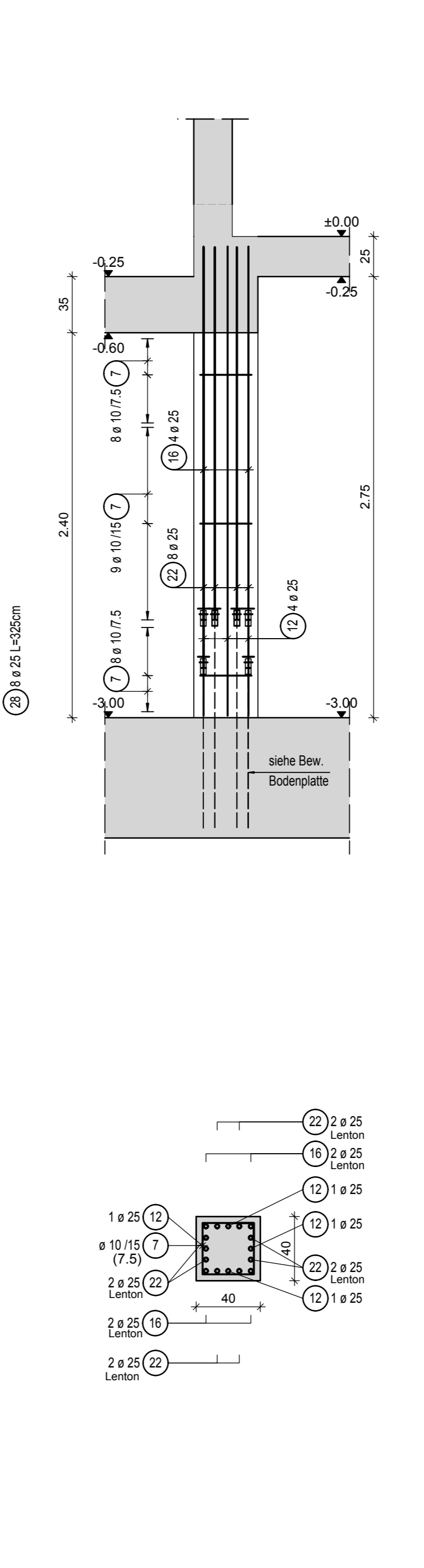
3x Stb. Stütze b/h=40/40cm (C35/45, XD3, XF1, WF) Pos. S39, Pos. S40, Pos. S41
