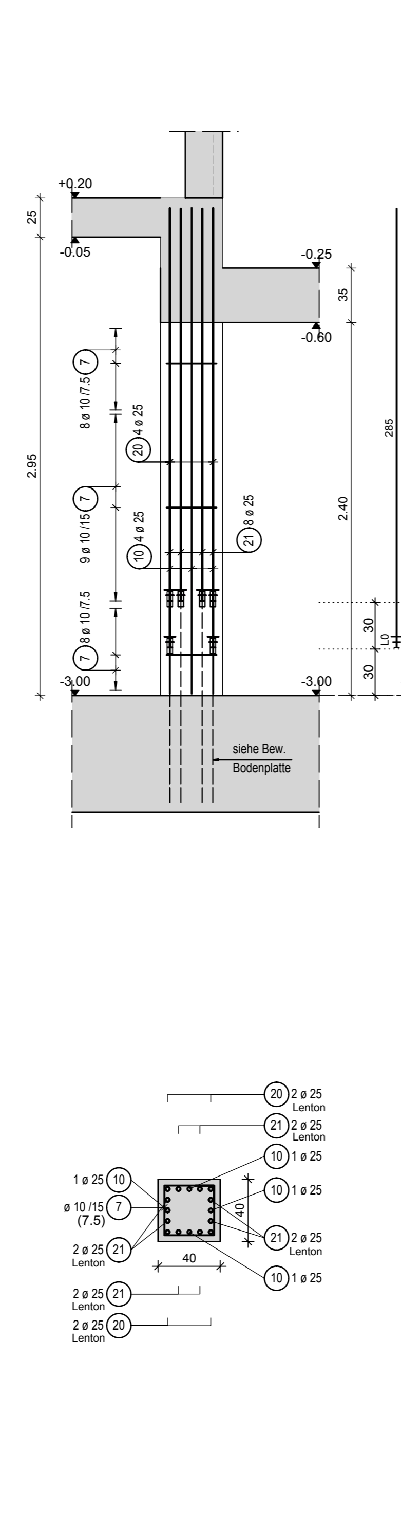
3x Stb. Stütze b/h=40/40cm (C35/45, XD3, XF1, WF) Pos. S46, Pos. S47, Pos. S48
