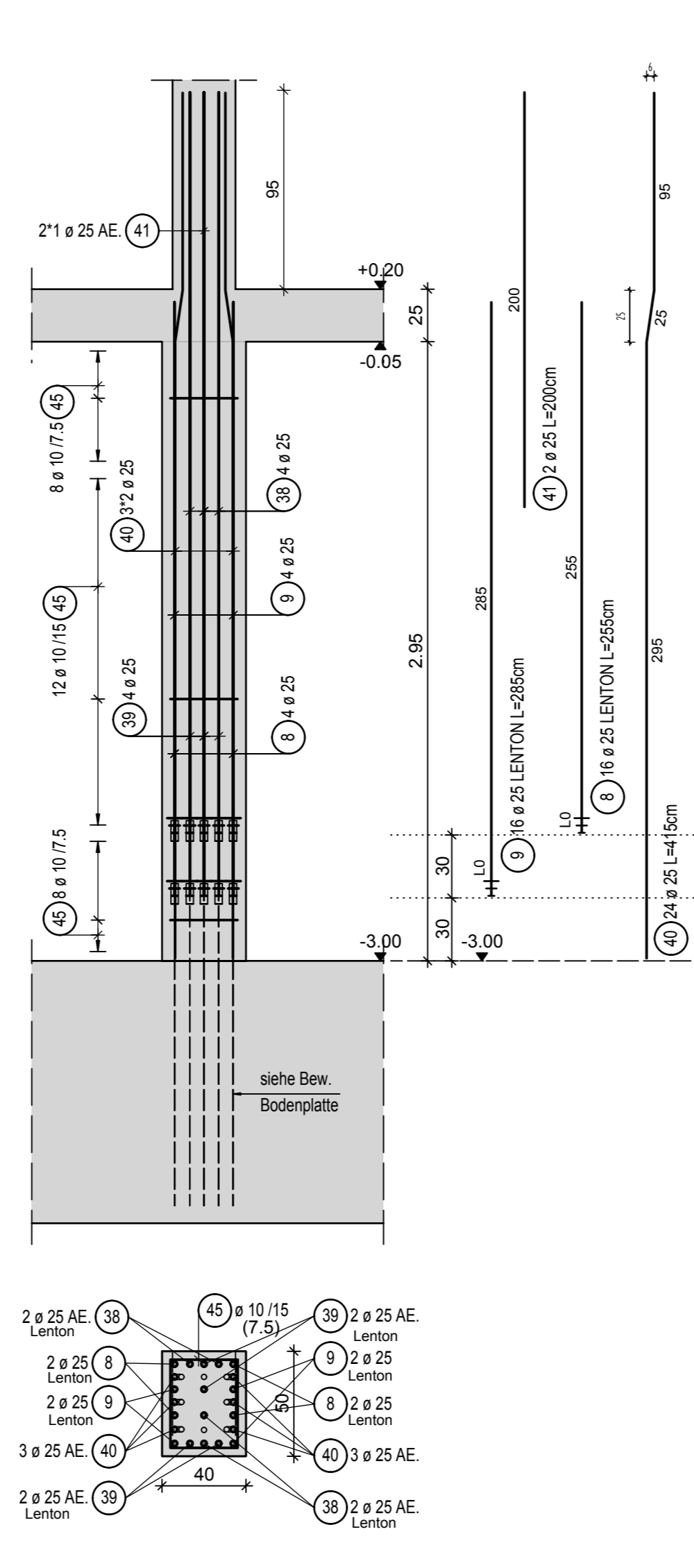
4x Stb. Stütze b/h=40/50cm (C35/45, XD3, XF1, WF) Pos. S49, Pos. S51 Pos. S52, Pos. S54
